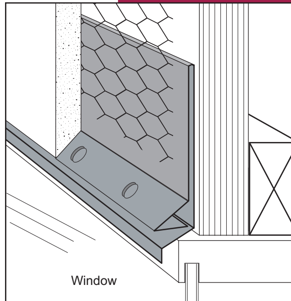
Typical Section, No Scale
